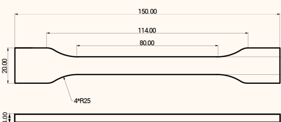
TENSILE TESTING SPECIMEN ISO 527
