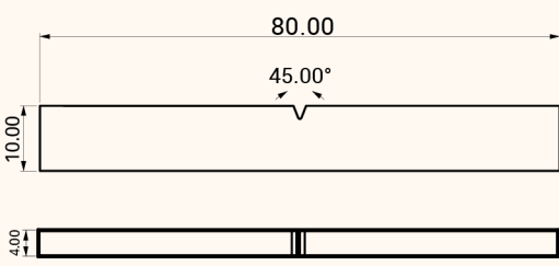
IMPACT TESTING SPECIMEN ISO 179
